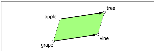
Figure 6.15 The parallelogram model for analogy problems (Rumelhart and Abrahamson, 1973): the location of \overrightarrow{vine} can be found by subtracting \overrightarrow{apple} from \overrightarrow{tree} and adding \overrightarrow{grape} .
